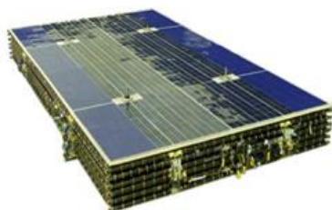
Figure 5. Stowed wing of the solar array
